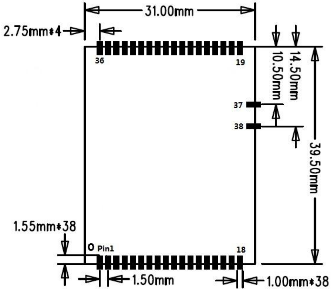
Figure 6-2 CWM630 module pin arrangement diagram (perspective view from the top of the module)
