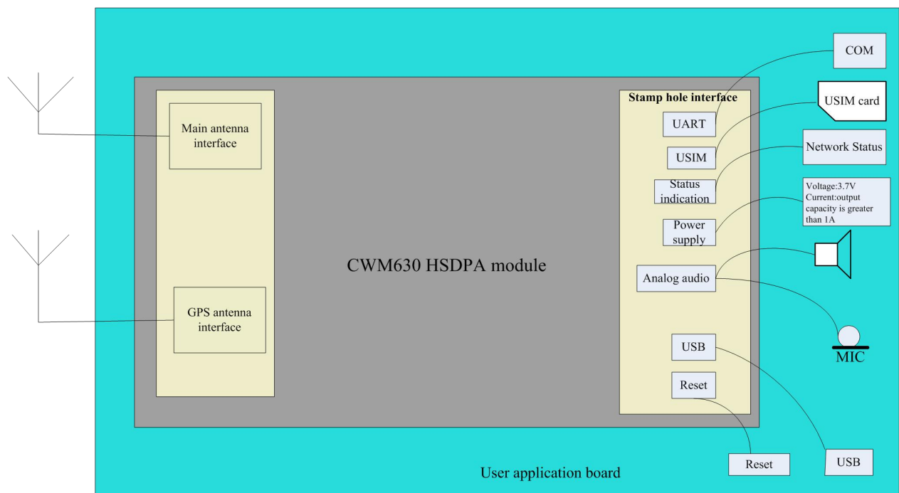
Figure 2-1 Functional Block Diagram of the CWM630 Module
