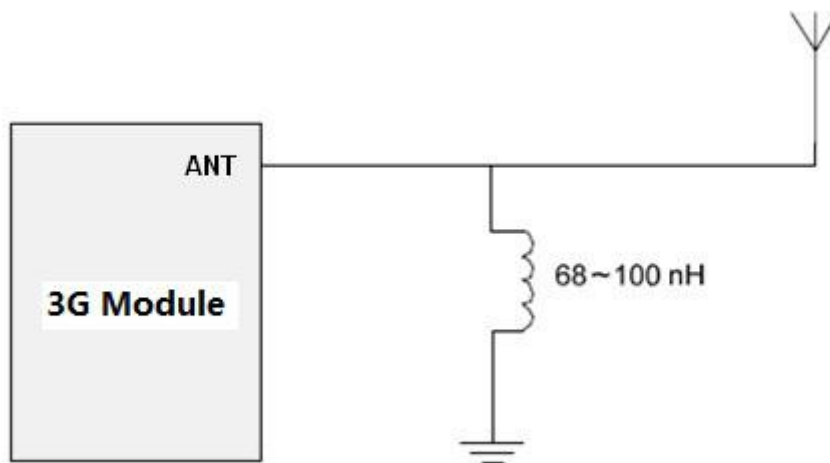
Figure 5-10 Antenna interface ESD protection recommende
