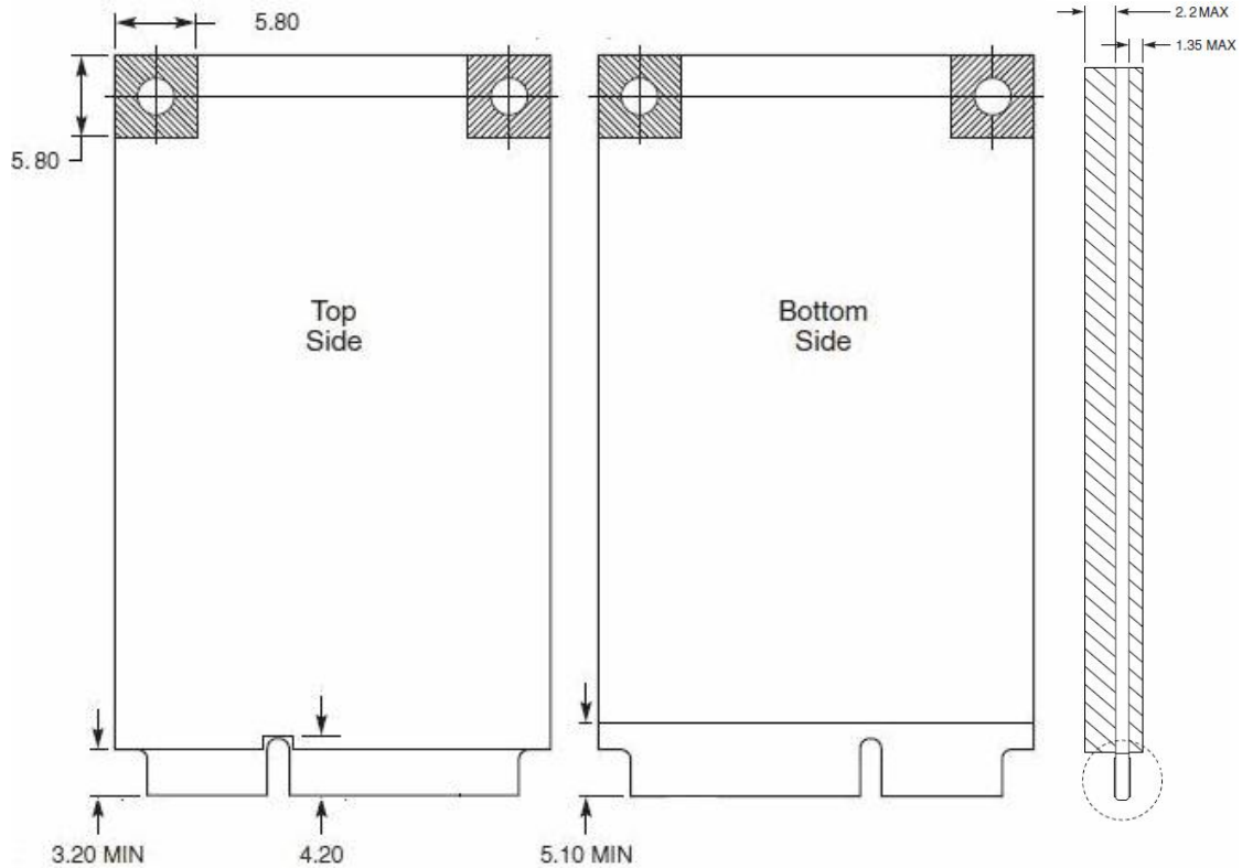
Figure 6-1 CWM600 series module structure size
