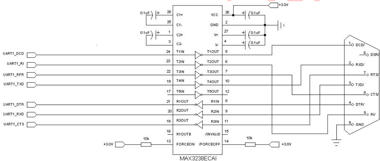
Figure 5-3 8-wire serial port reference design
