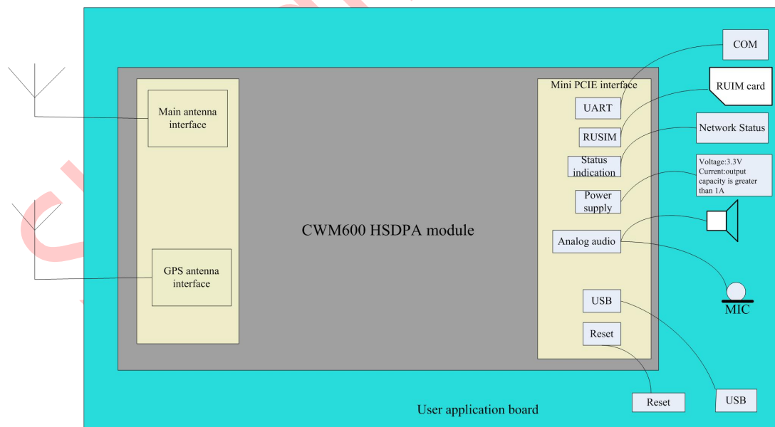
Figure 2-1 CWM600 module block diagram
