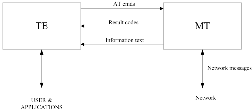
Figure 1-1 AT command interface
